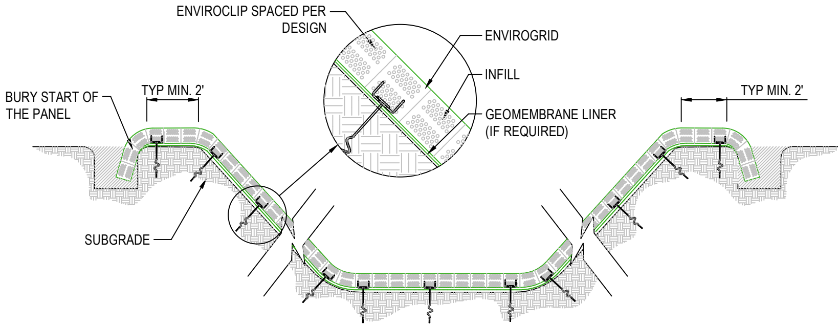
CROSS SECTION
