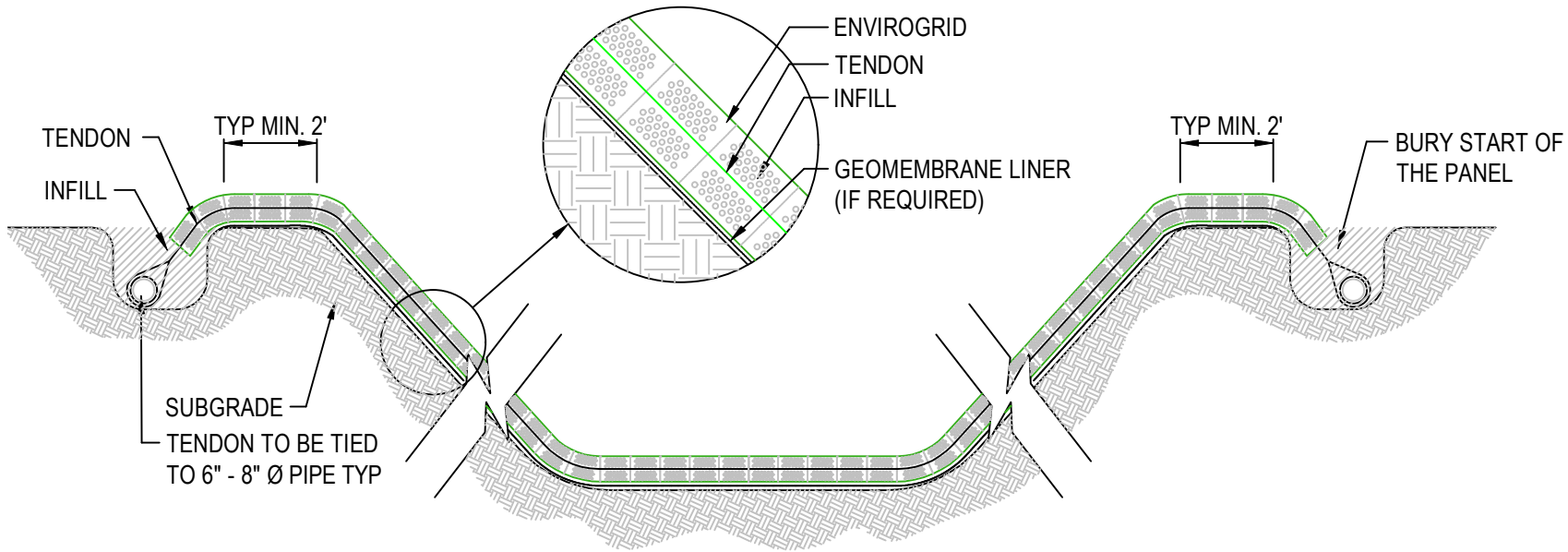
CROSS SECTION
