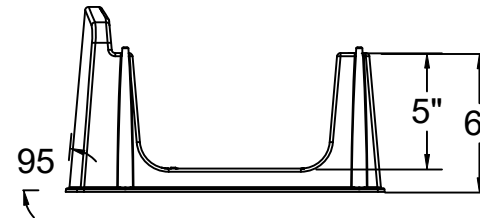
SIDE VIEW WITHOUT SIDE RAILS
